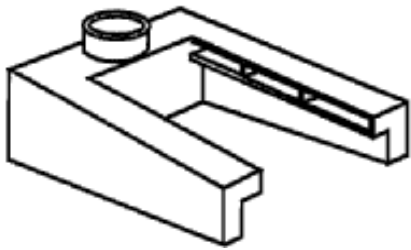
Double Lateral Hood Lengths from 24" to 96" Widths from 18" to 66"
